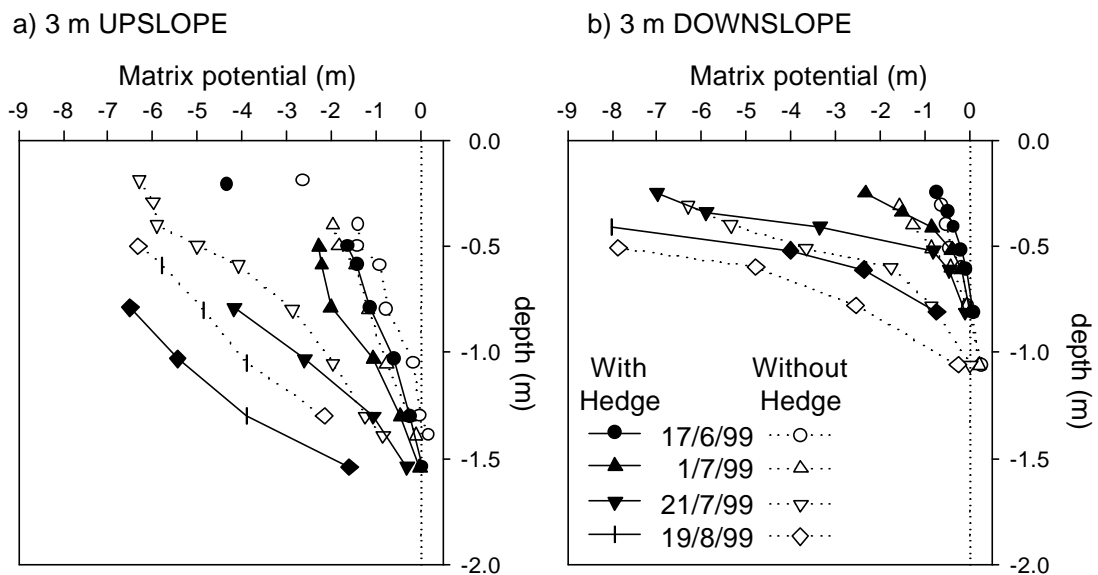
Figure 6 : Profiles of soil matrix potential at 3 m a) upslope and b) downslope from the transects in summer 99.
