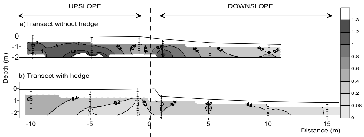
Figure 4 : Contour lines of groundwater nitrate level the 11 th of February 1999 along the transect without hedge (a) and with hedge (b). Crosses represent the sampling points.
