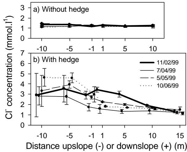
Figure 3 : Evolution of groundwater chloride level along the transect without hedge (a) and with hedge (b). Mean and standard deviation of each piezometer.
